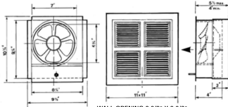
WALL OPENING 9 3/8" X 8 3/8"
